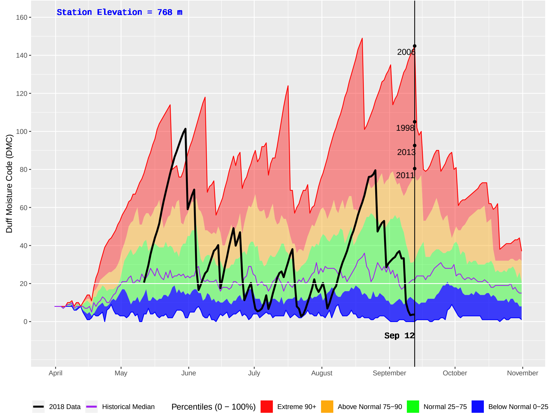
GRAHAM (124) : Historical (1979–2016) and Current (2018) Daily Duff Moisture Code (DMC)
