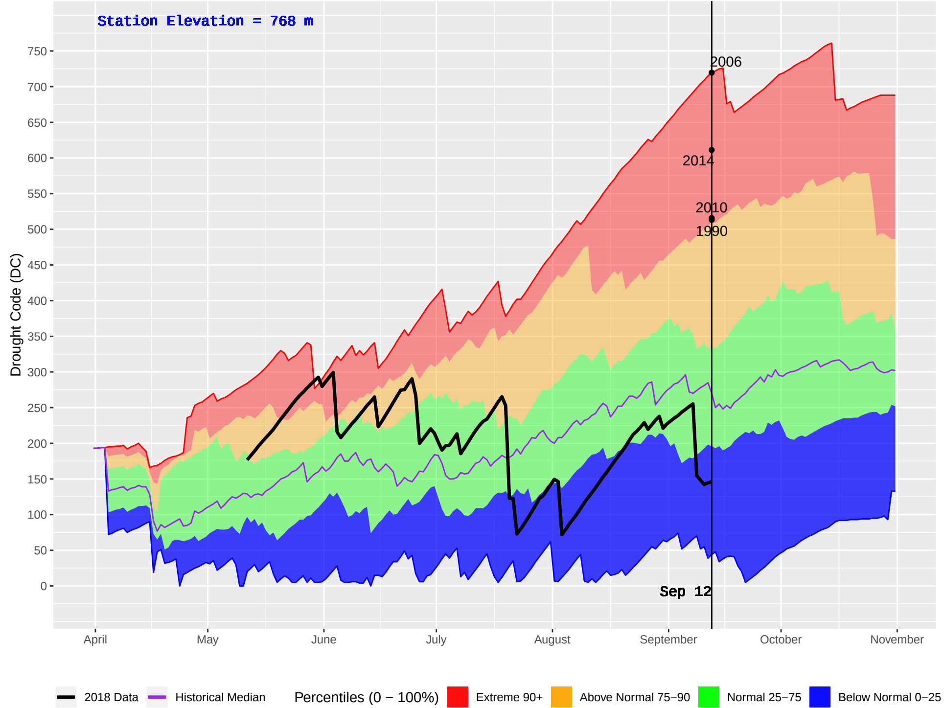
GRAHAM (124) : Historical (1979–2016) and Current (2018) Daily Drought Code (DC)
