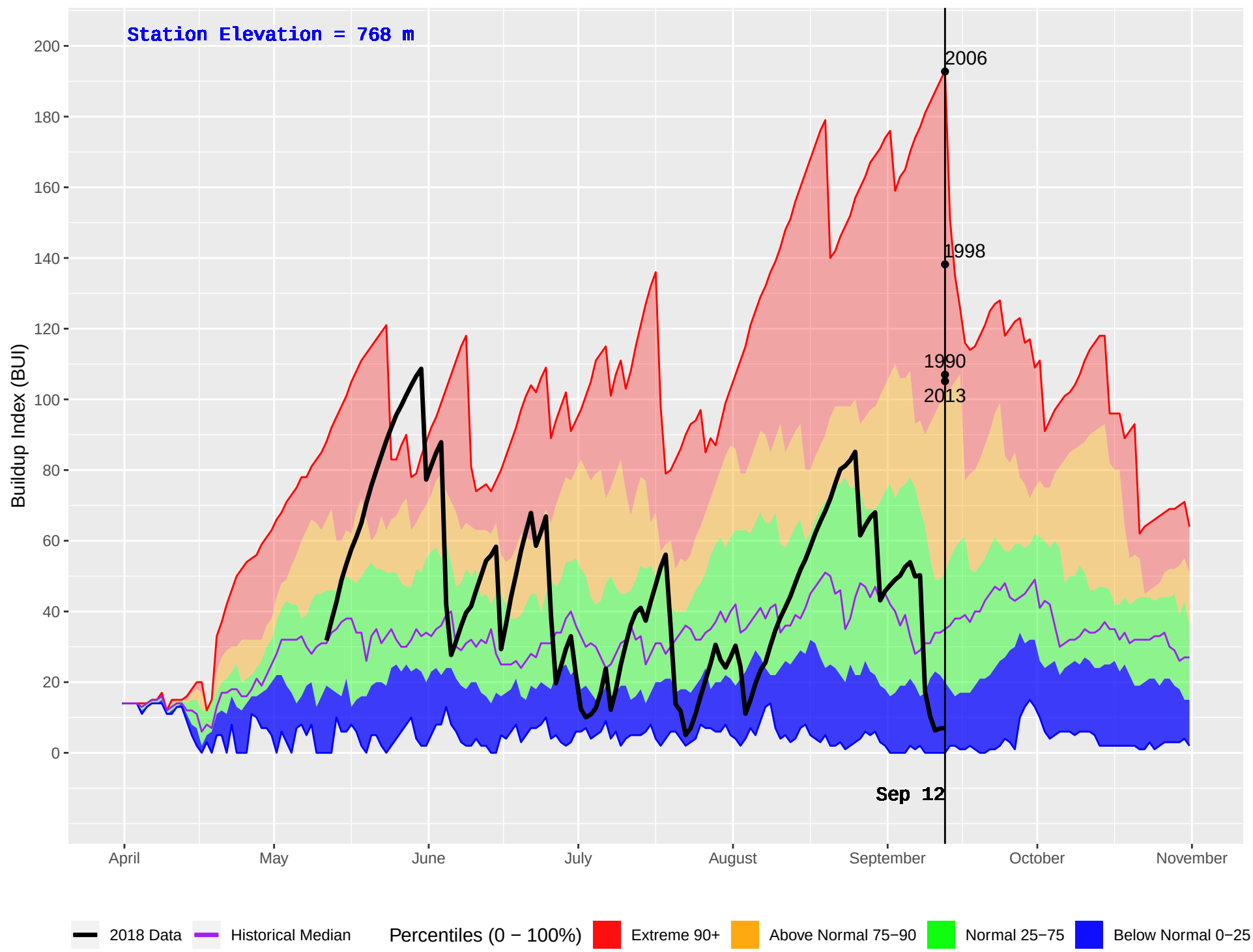
GRAHAM (124) : Historical (1979–2016) and Current (2018) Daily Buildup Index (BUI)
