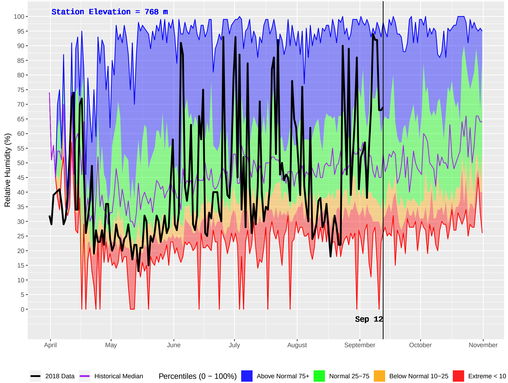
GRAHAM (124) : Historical (1979–2016) and Current (2018) Daily Relative Humidity
