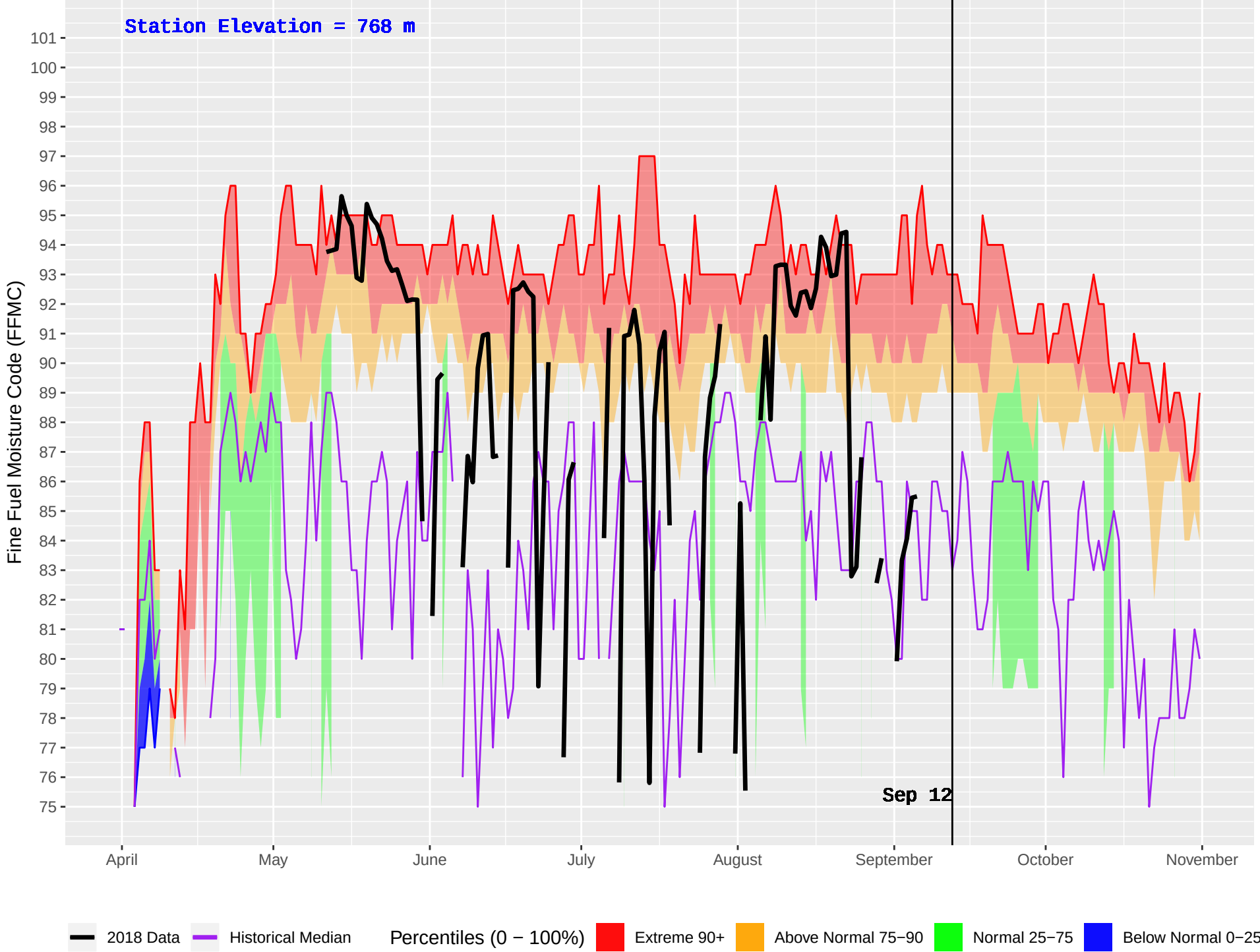
GRAHAM (124) : Historical (1979–2016) and Current (2018) Daily Fine Fuel Moisture Code (FFMC)
