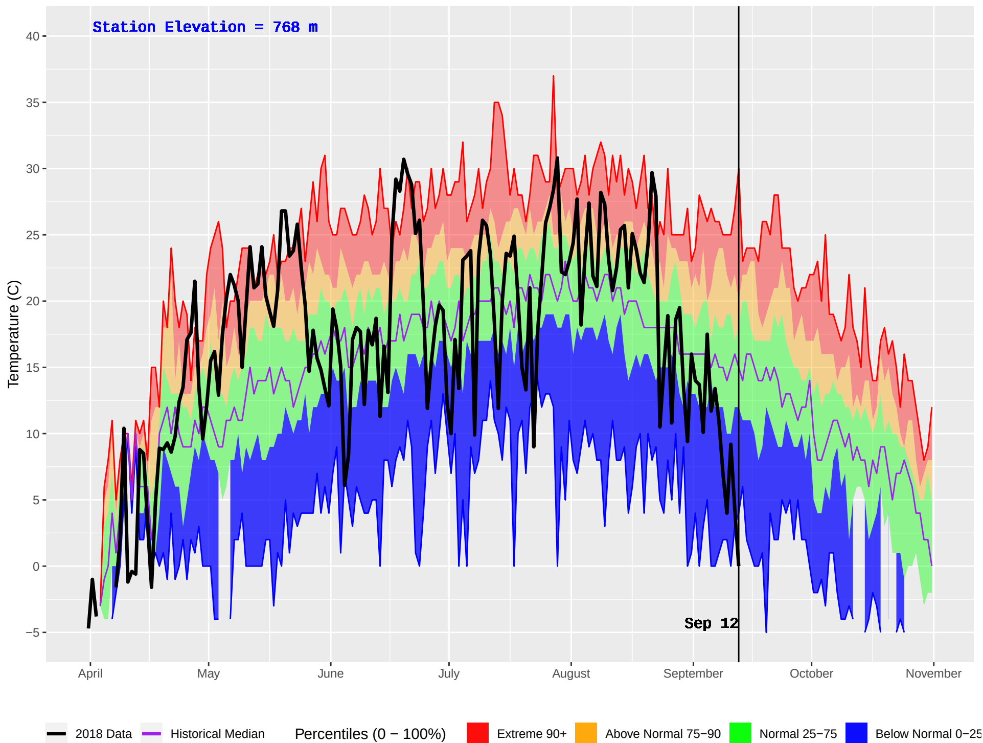
GRAHAM (124) : Historical (1979–2016) and Current (2018) Daily Temperature
