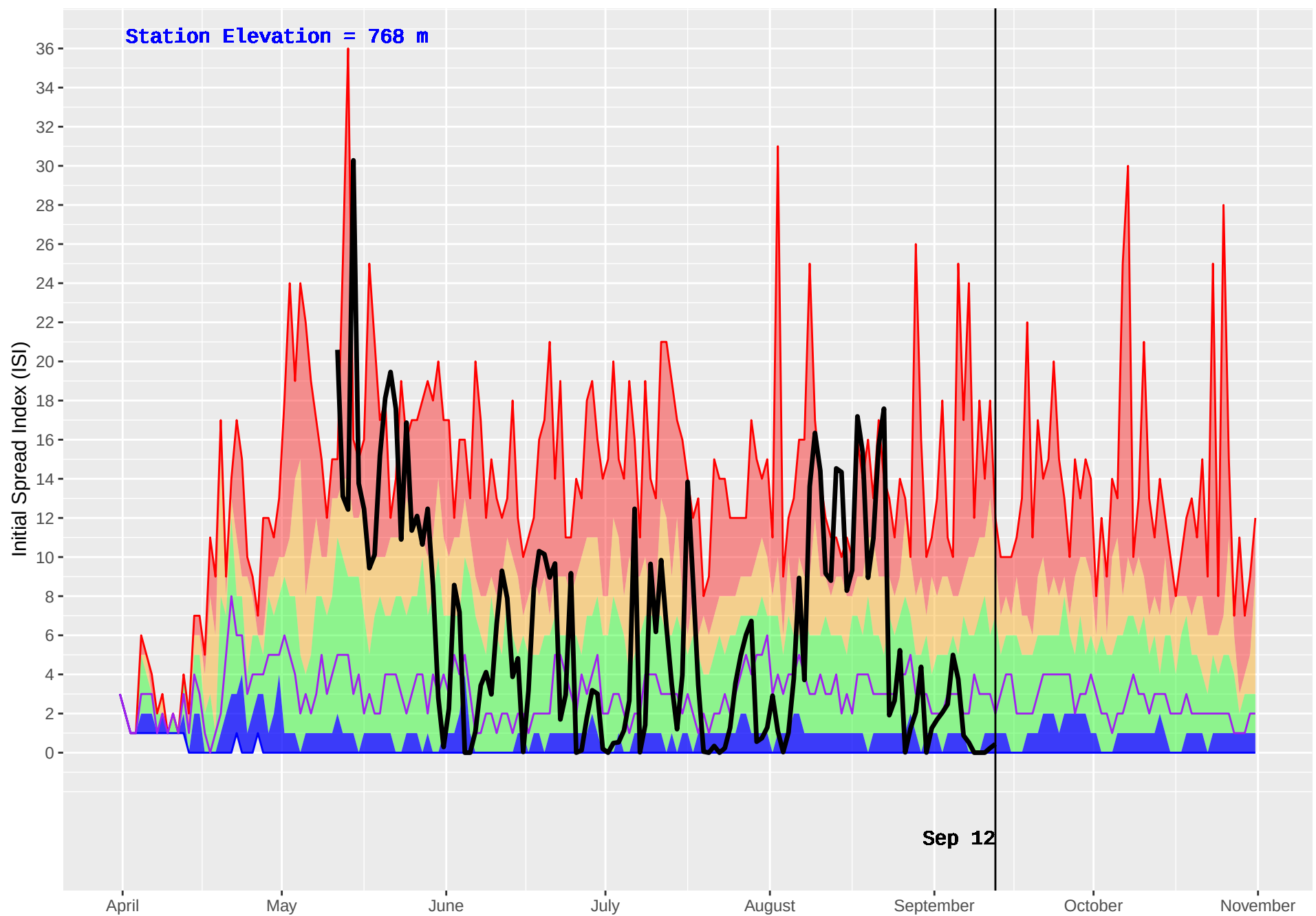
GRAHAM (124) : Historical (1979–2016) and Current (2018) Daily Initial Spread Index (ISI)
